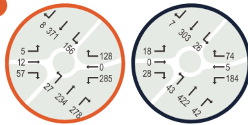
Proposed Roundabout
