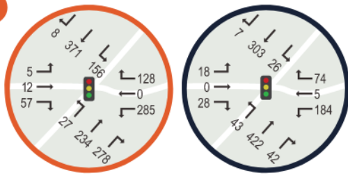
Proposed Signal
