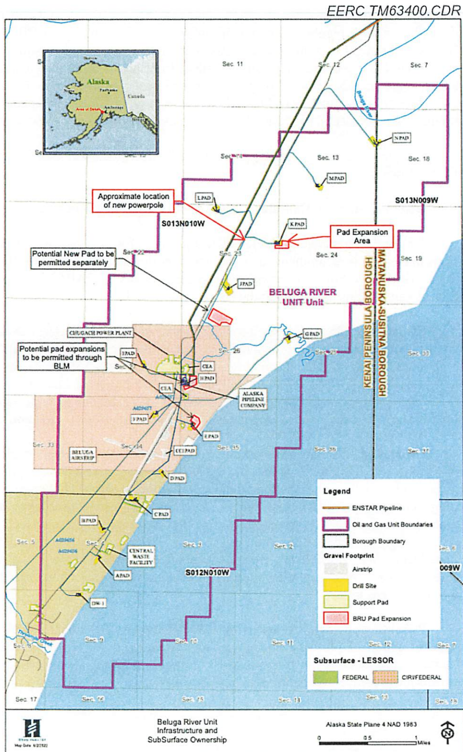
Figure 15. Beluga River Unit Infrastructure and Subsurface Lease Ownership (Alaska Department of Natural Resources, 2022b).
