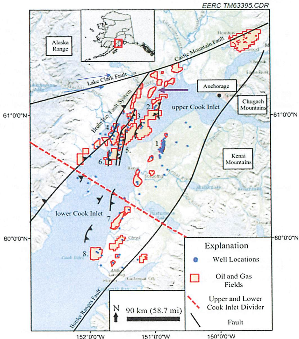
Figure 10. Location Map of Cook Inlet Basin with Beluga River Field Indicated by Purple Arrow (Pantaleone and Bhattacharya, 2021)
